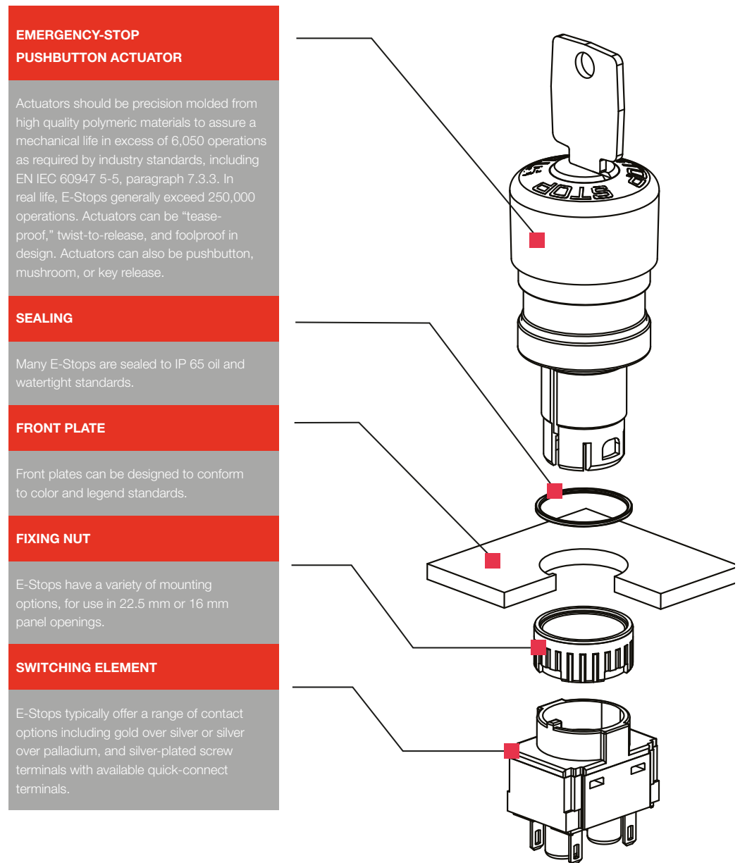
Figure 1 – Parts of an E-Stop
