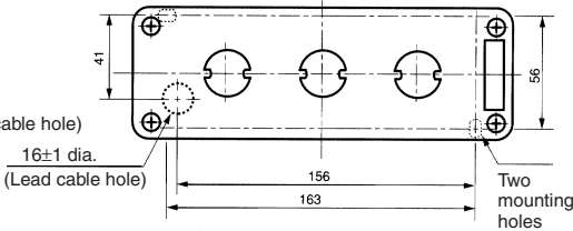
Cable Port Hole (Top View)
