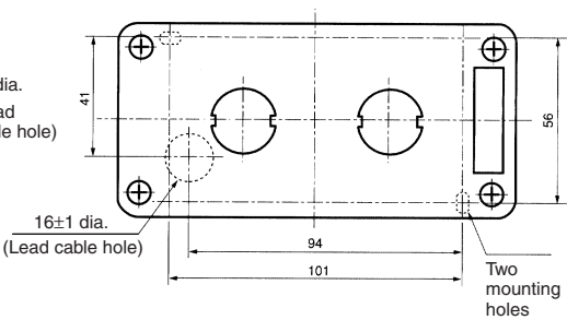
Cable Port Hole (Top View)
