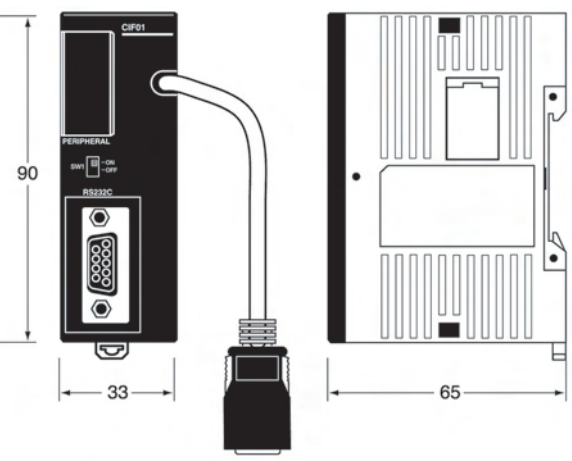
Peripheral/RS-232C Adapter Unit (CPM2C-CIF01-V1)
