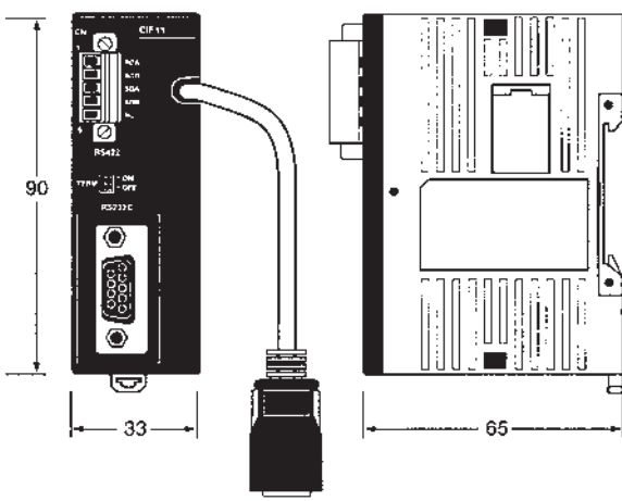
RS-422/RS-485/RS-232C Adapter Unit (CPM2C-CIF11)
