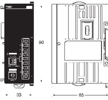
Temperature Sensor Unit (CPM2C-TS001, CPM2C-TS101)
