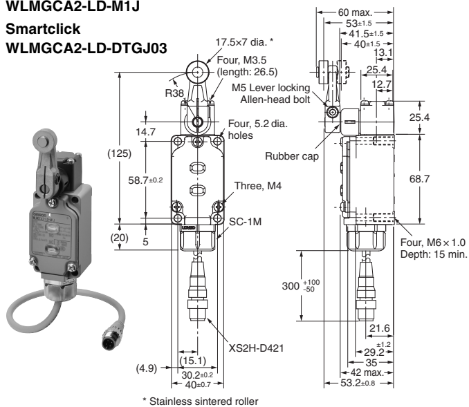
* Stainless sintered roller Note: The photo shows the WLMGCA2-LD-M1J model.
