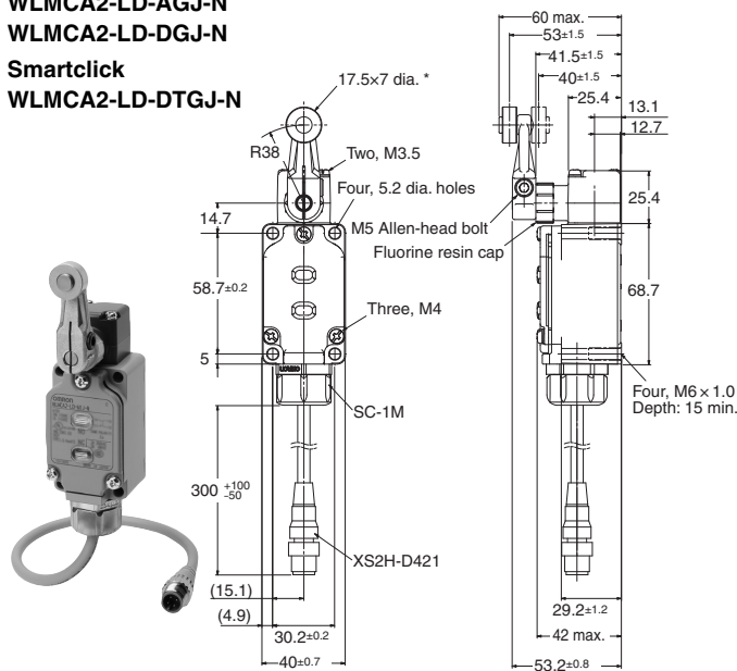
* Stainless sintered roller Note: The photo shows the WLMCA2-LD-M1J-N model.
