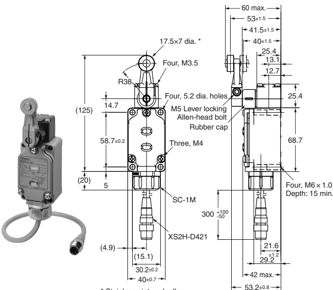
* Stainless sintered roller Note: The photo shows the WLMG2-LD-M1J model.
