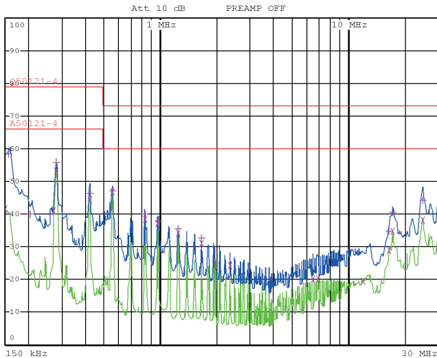
Fig. 8a XRCM60-24: Typ. disturbance voltage at the input ( V_i = 16.8\text{ V} , I_{i, nom} , resistive load, quasi peak and average)
