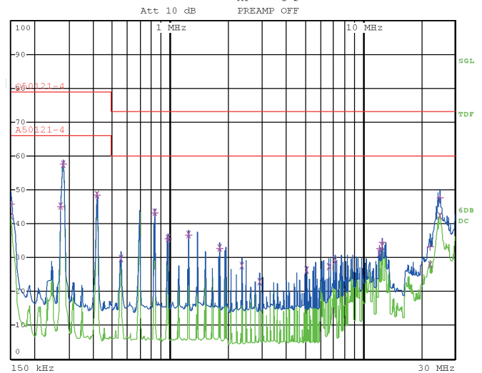
Fig. 8b XRCM60-24: Typ. disturbance voltage at the input ( V_i = 137.5\text{ V} , I_{i, nom} , resistive load, quasi peak and average)
