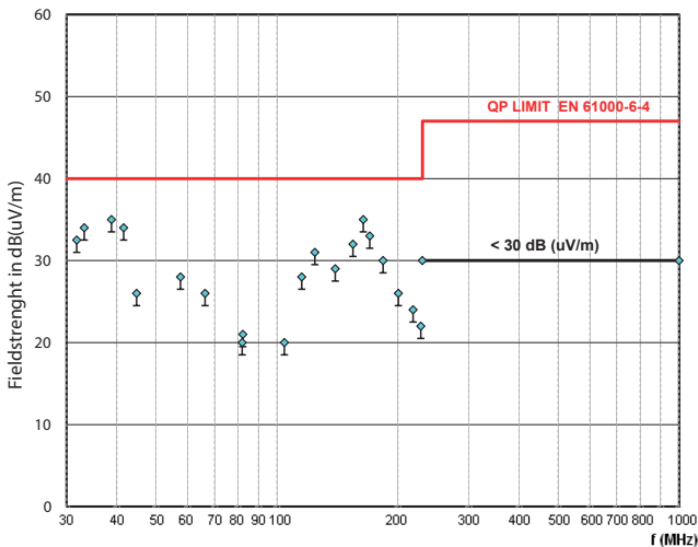
Fig. 9a XRCM60-24: Typ. radiated disturbances in 10 m distance ( V_i = 16.8\text{ V} , I_{i, nom} , resistive load, quasi peak).
