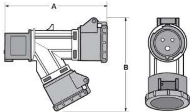
A:160 B:168 Dimensions in mm
