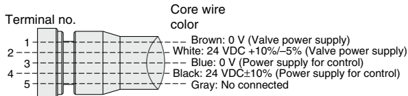
Connections (PROFIBUS DP)
