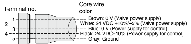
Connections (DeviceNet™)
