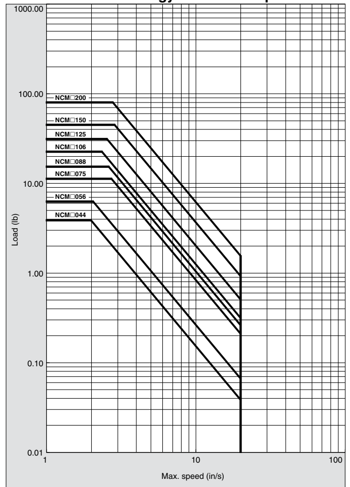
Graph (4) Allowable Kinetic Energy without Bumper
