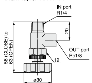
Drain valve: VBAT-V1
