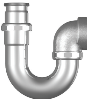
AP250-017 Chrome Plated Cast Brass Tailpiece and Trap. 1 1/4" NPT male inlet, 1 1/2" NPT female outlet.
