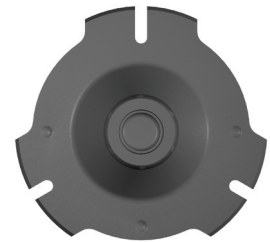
150-032 Powder Coated Cast Aluminum Floor Flange. 1 1/4" NPT female thread.
