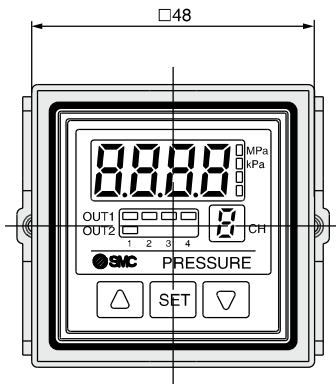
□48 conversion adapter + Panel mount adapter
