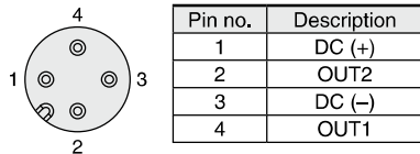
Power supply/output connector pin no.
