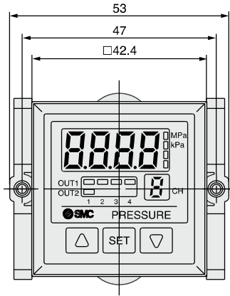
Front protective cover + Panel mount adapter
