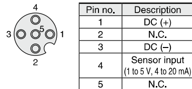
Sensor connector pin no.
