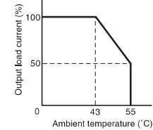
Relationship between Output Load Current and Ambient Temperature (CP1W-16ER/32ER)
