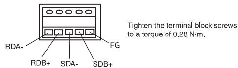
RS-422A/485 Connector
