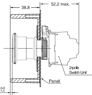
Push-in Plus Terminal Block Type Mounting a 2-pole Switch Unit
