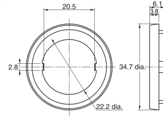
30-dia. Resin Attachment A22Z-A30
