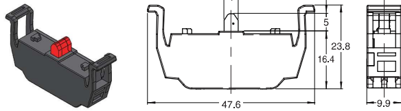
Switch Block (one contact) A22NZ-S-P1□
