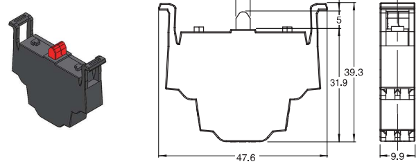
Mounting Latches A22NZ-H-02
