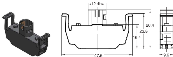
Lighting unit A22NZ-T-□P
