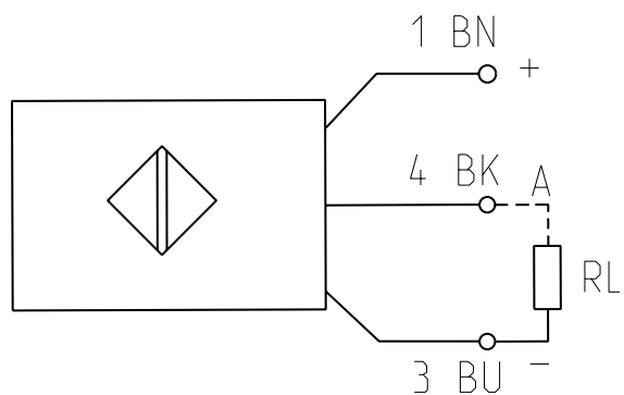
Contact diagram
