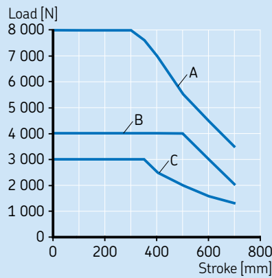
Push load reduction static Safety factor S=2
