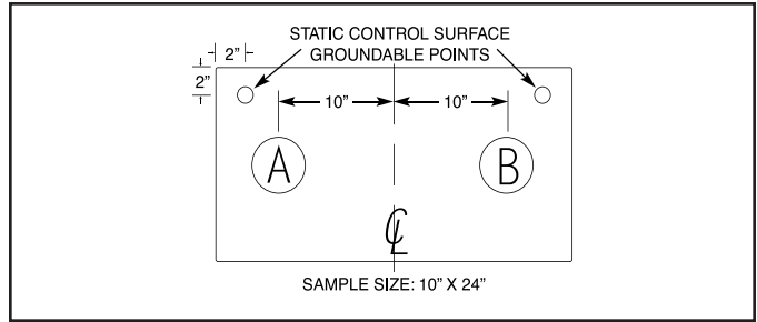
Figure 6. Material Evaluation Sample Configuration.
