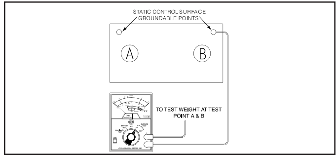
Figure 7. Material Evaluation Surface to Groundable Point Test.
