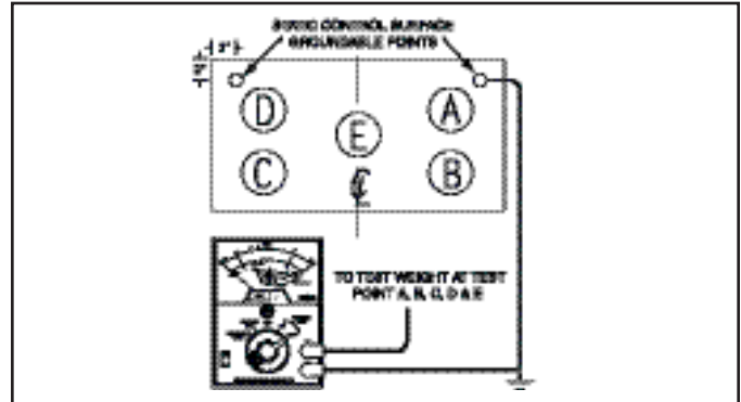
Figure 4. Periodic Performace Tests of Installed Surfaces.
