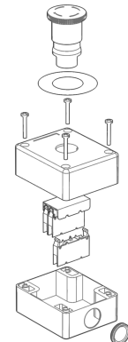
Figure 1. Assembly
