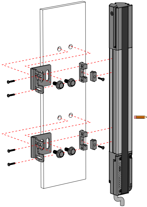
Figure 19. Side-Mount Brackets
