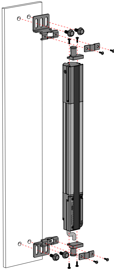
Figure 17. End-Mount Brackets
