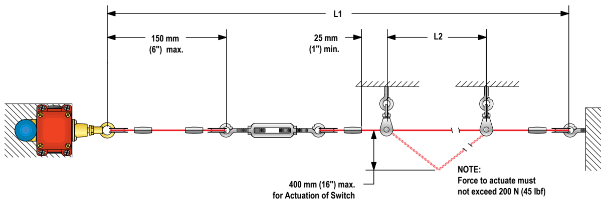
Figure 2. Assembly of Rope and Hardware
