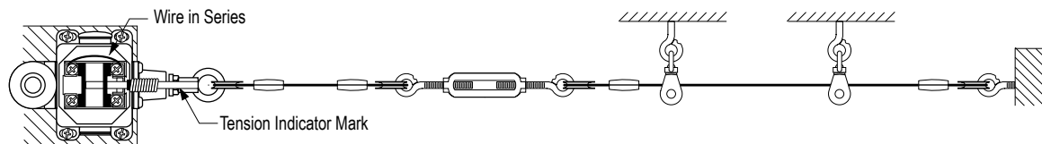
Figure 3. Run Position: Proper Rope Tension
