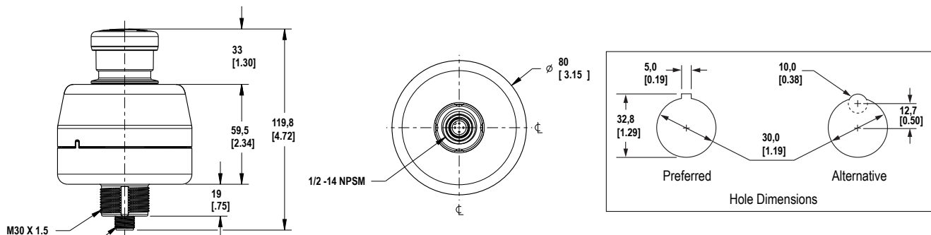
Figure 2. Standard 40 mm Pushbutton
