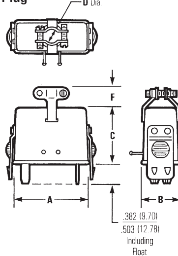
Plug
