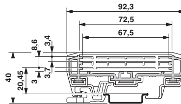
Dimensional drawing
