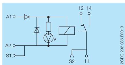
RB(R)121P(G)-5VDC/12VDC
