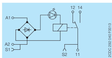
RB(R)121(G)-48-60VUC/ 115VUC/230VUC/60-230VUC
