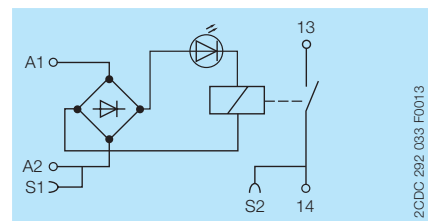
RB111-115VUC/230VUC
