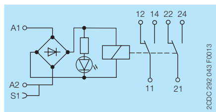
RB(R)122G-24VUC/48-60VUC
