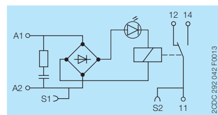
RB(R)121R-115VUC/230VUC
