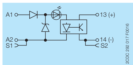
OB(R)IC0100-5-12VDC OB(R)OC2000-5-12VDC
