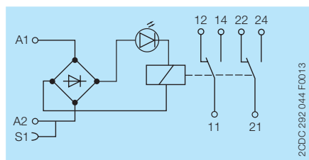
RB(R)122G-115VUC/230VUC
