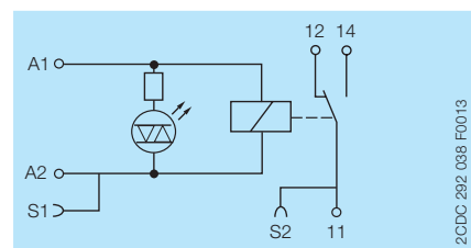
RB(R)121-12VDC/24VDC
