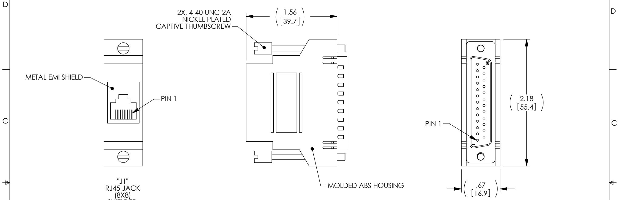
"P1" 25 PIN MALE D-SUB CONNECTOR
