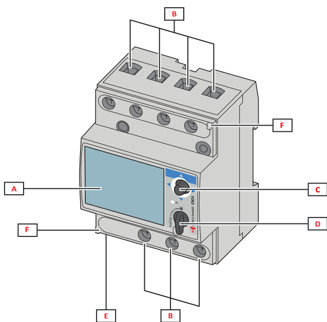
Fig. 1 Direct connection
