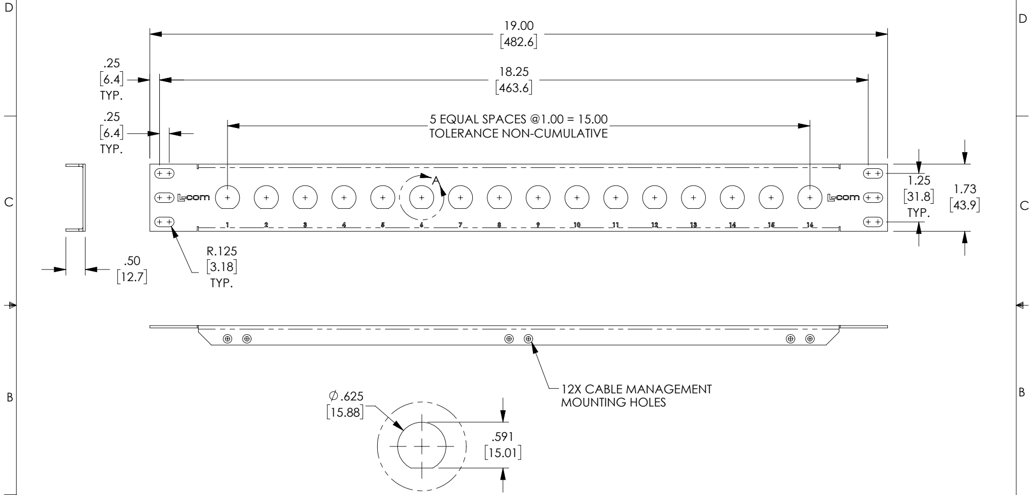
DETAIL A SCALE 2 : 2.5
