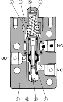
Non-actuated
