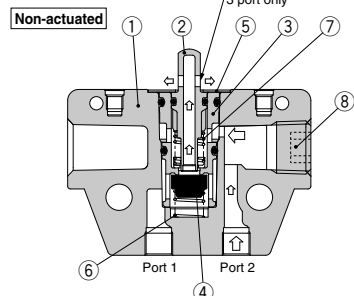
Bottom ported
