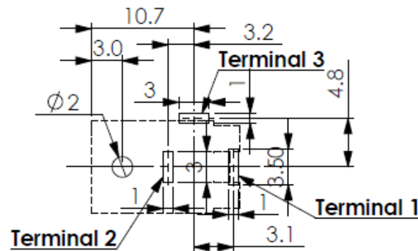
RECOMMENDED P.C.B. LAYOUT (BOTTOM VIEW)
