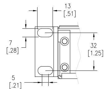
VIEW D (MOUNTING BRACKET-ENLARGED)
