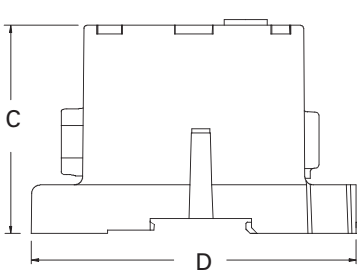
Loadside
