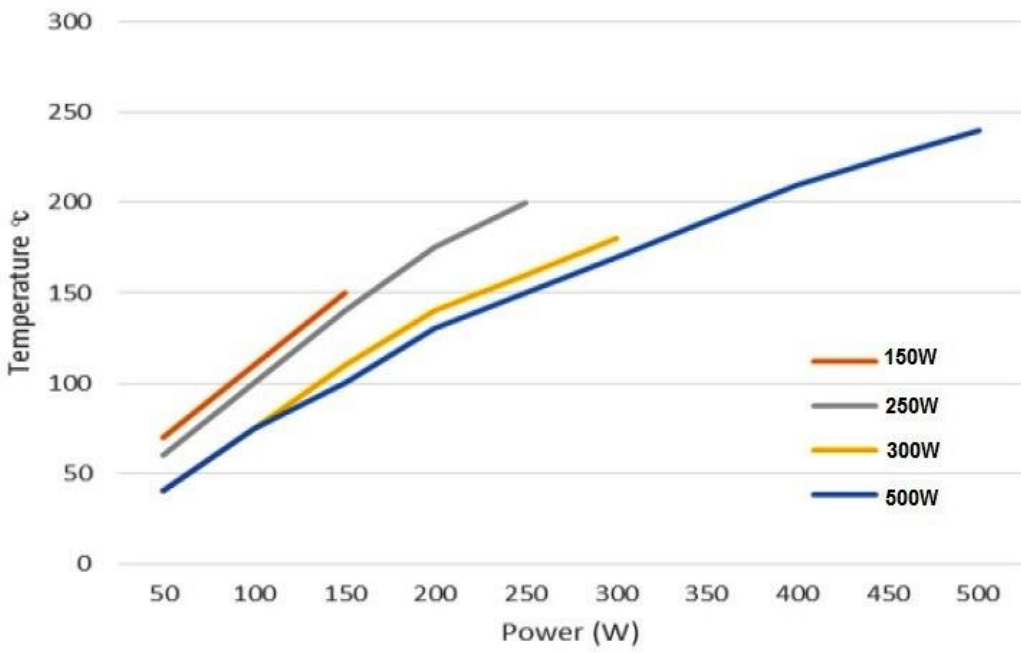
Typical Surface Temp Vs Power
