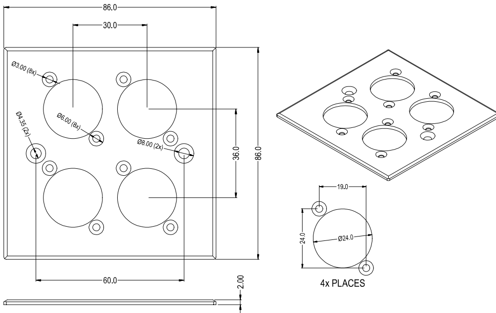
RS30500 - 4 WAY FACEPLATE - PLAIN
