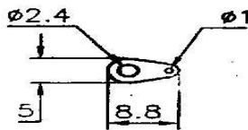
SOLDER TERMINAL
