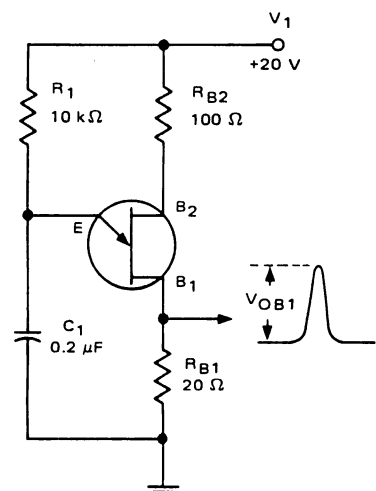
FIGURE 3 - V_{OB1} TEST CIRCUIT (Typical Relaxation Oscillator)
