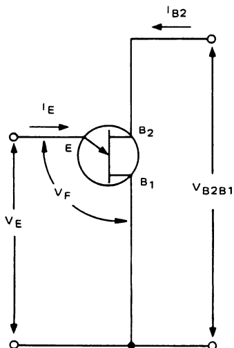
FIGURE 1 UNIUNION TRANSISTOR SYMBOL AND NOMENCLATURE
