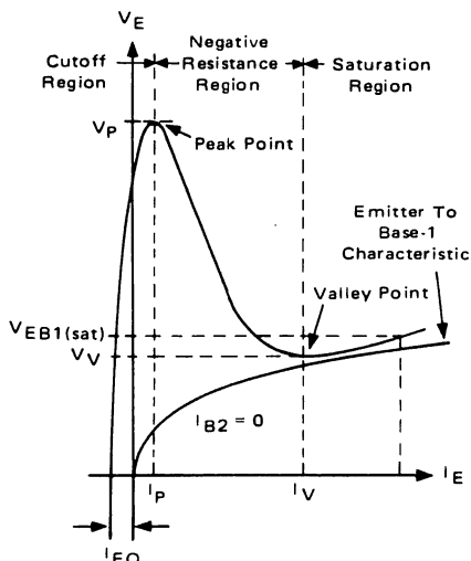
FIGURE 2 STATIC EMITTER CHARACTERISTIC CURVES
