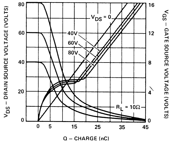
FIGURE 10. Turn-on Charge
