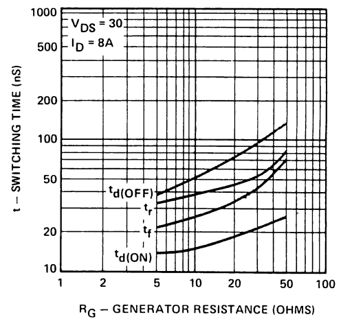
FIGURE 9. Effects of Drive Resistance
