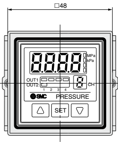
□48 conversion adapter + Panel mount adapter
