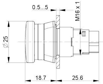
Dimensioned drawing
