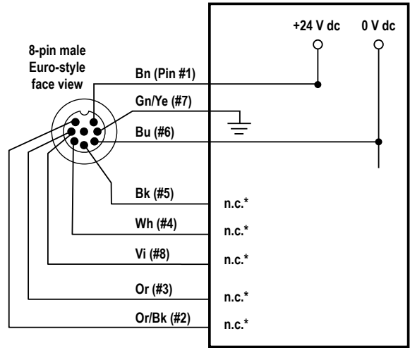
Figure 29. Emitter—Generic hookup
