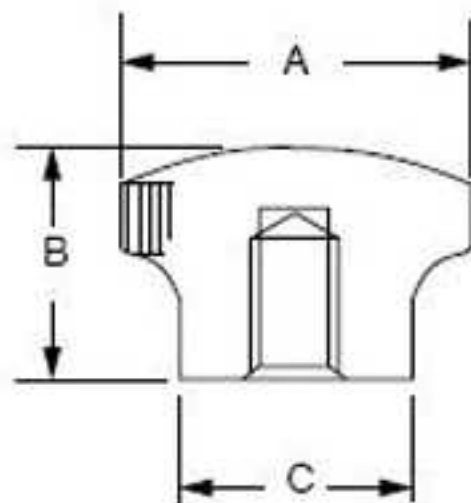
Molded Thread
