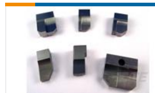
TE Model / Part #8-240655-8 ANVIL
