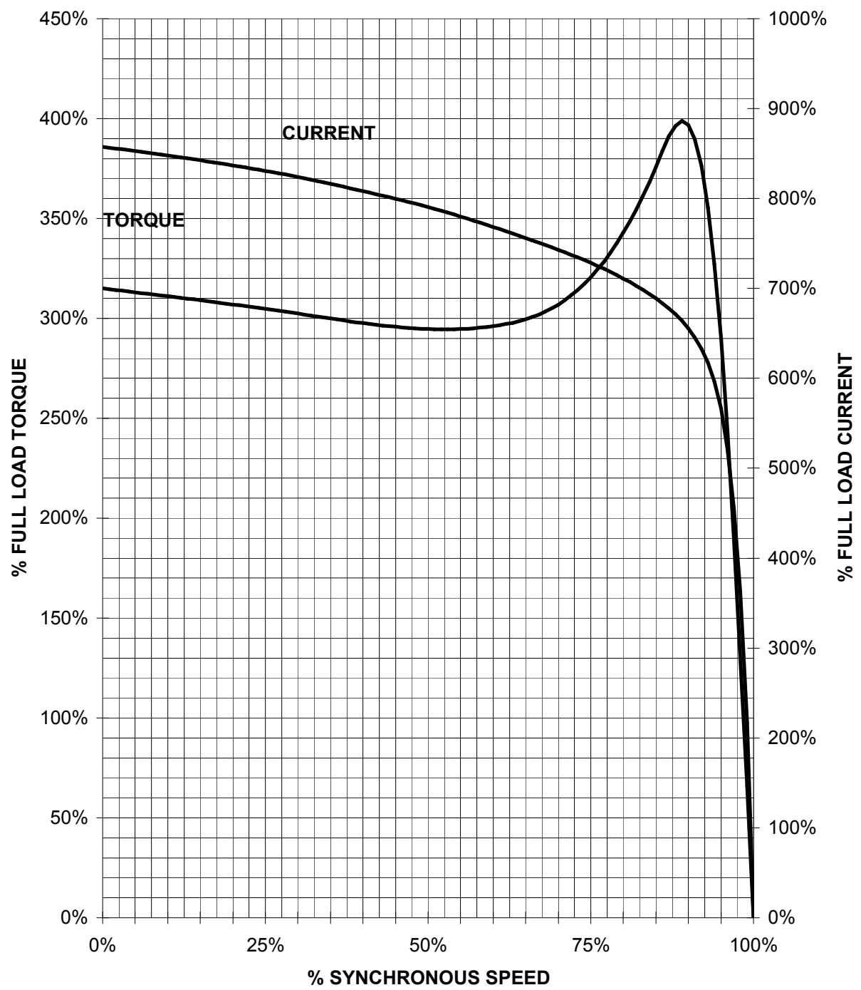
TORQUE & CURRENT VS. SPEED
