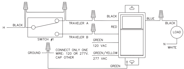
WIRING DIAGRAM: 3 WAY INSTALLATION SS703Z CONNECT A WIRE INSIDE THE GANG-BOX BETWEEN TRAVELER A AND HOT
