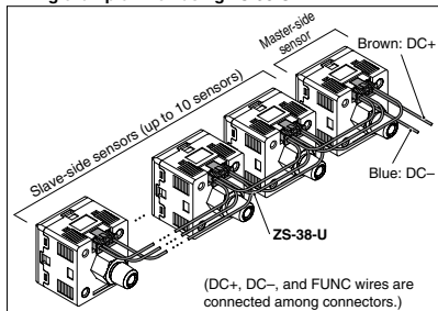
Wiring example when using ZS-38-U
