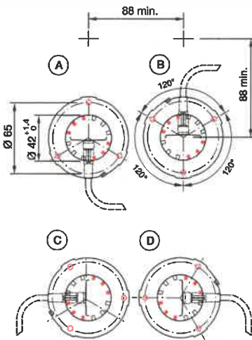
Mounting cut-outs [mm]
