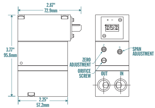
Figure 7: Terminal Block
