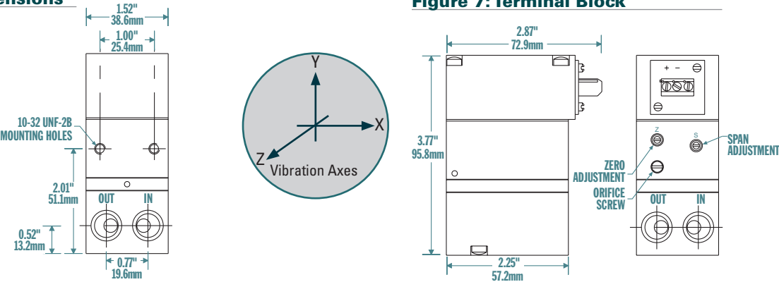
Back Dimensions
