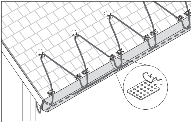
Figure 7. Standard roof clip attachments
