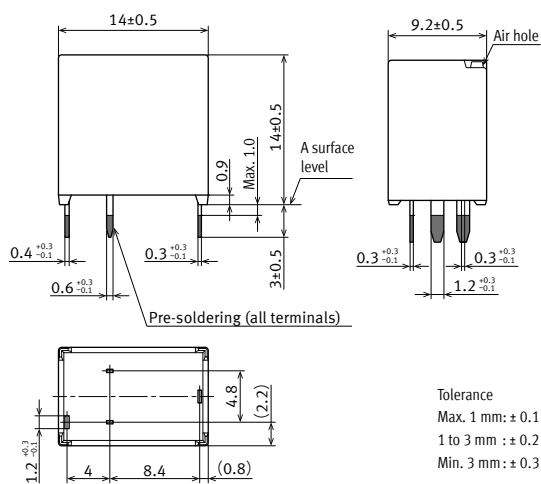
External dimensions
