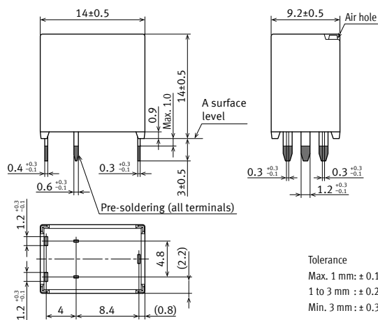
External dimensions
