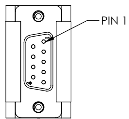
"P1" 9 PIN MALE D-SUB CONNECTOR
