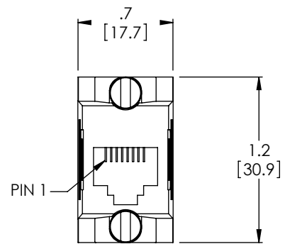
"J1" RJ45 JACK (8X8)
